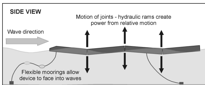
Fig. 7. Side view of Pelamis wave energy converter, adapted from [18].
