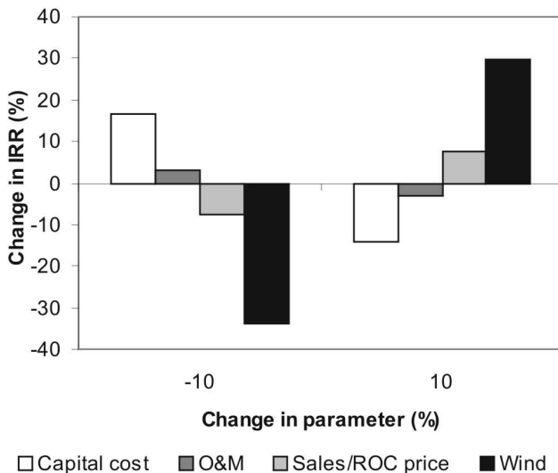
Fig. 12. Sensitivity of IRR to key project variables
