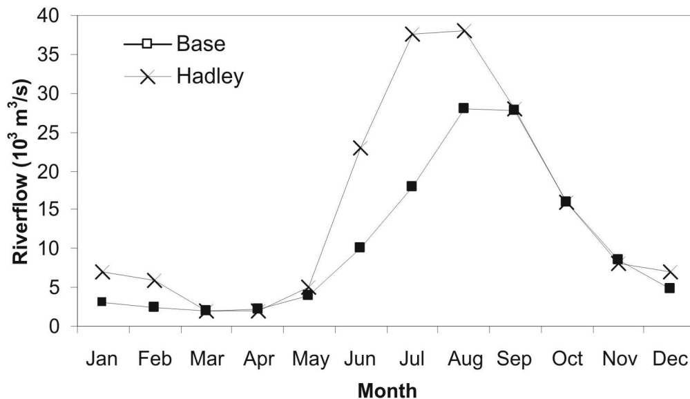
Figure 4. Historic (Base) and projected river flows at location in Lower Mekong Basin for Hadley Centre scenario (adapted from [7])
