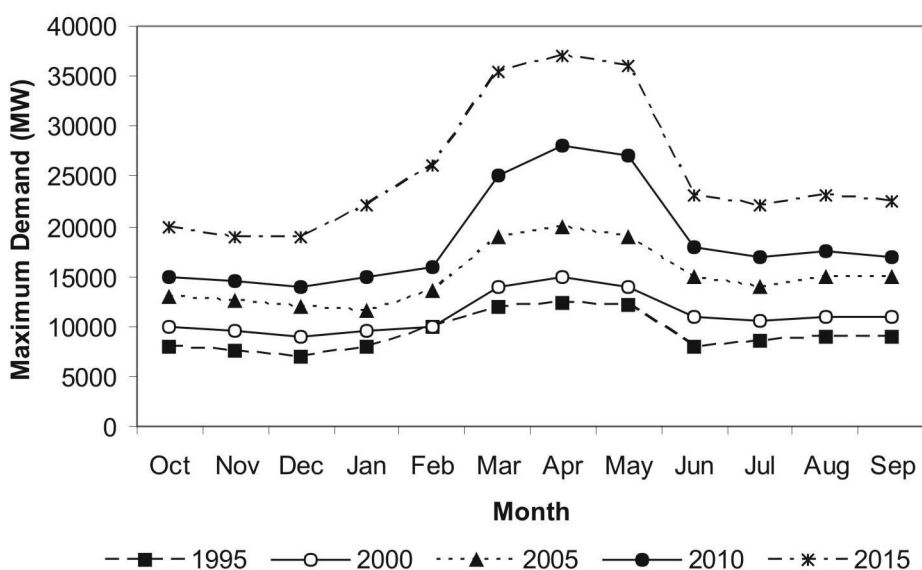
Figure 8. Maximum electricity demand curves for Thailand [13]
