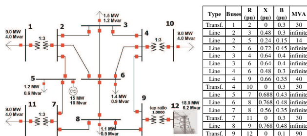
Figure 4. 12-bus 14-line test case and transformer/line characteristics
