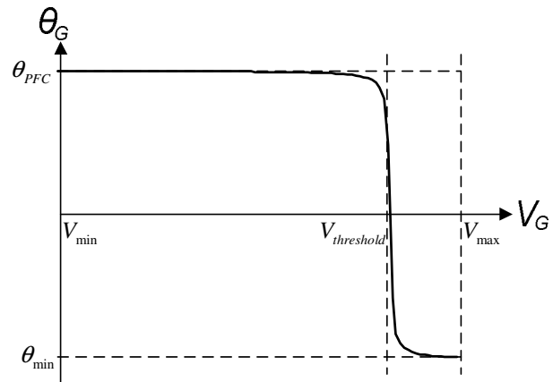
Figure 3. Smoothing of control strategy transition for Intelli-Gens.
