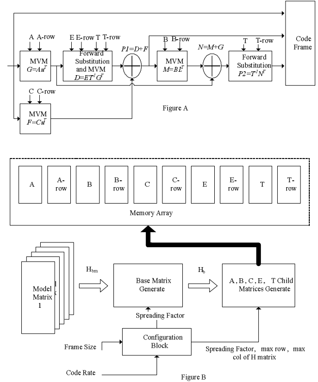
Figure 1: (Real Time Programmable LDPC Encoder)
