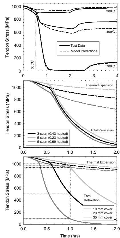
Figure 5: (a) Observed and predicted prestress relaxation for a locally-heated tendon and (b) effect of heated length ratio and (c) concrete cover at midspan on prestress relaxation during heating at 10°C/min to a predetermined temp.
