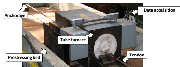
Figure 3: Localized heating relaxation tests on stressed tendons
