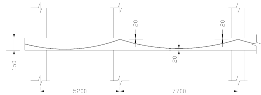
Figure 4: Example flat plate UBPT Structure used in analyses
