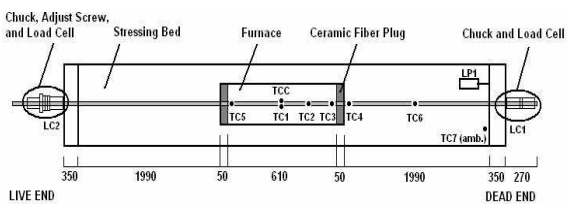
Figure 2: Relaxation test setup
