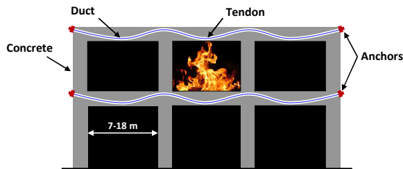
Figure 1: Single bay fire in a multi-bay structure
